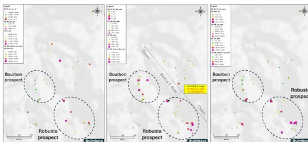
Figure 2. Preliminary geochemistry: the first two prospects have been identified in the property related with high mineralisation of copper/molybdenite and epithermal gold veins.
