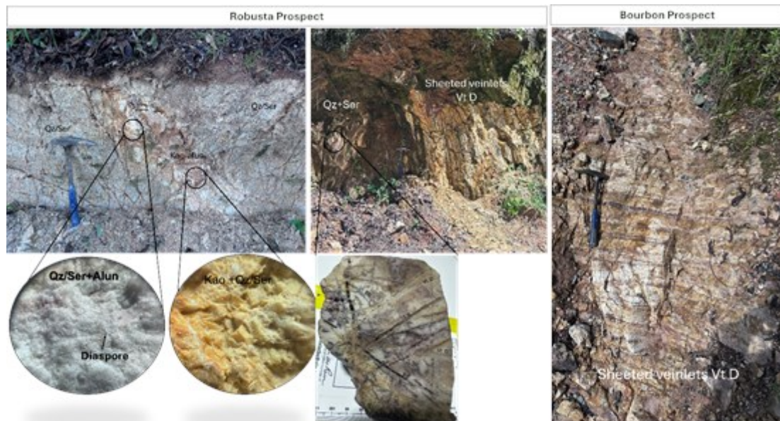
Figure 4. Porphyry Footprint outcrops with strong Advance Argillic alteration and quartz-sericitic alteration.
